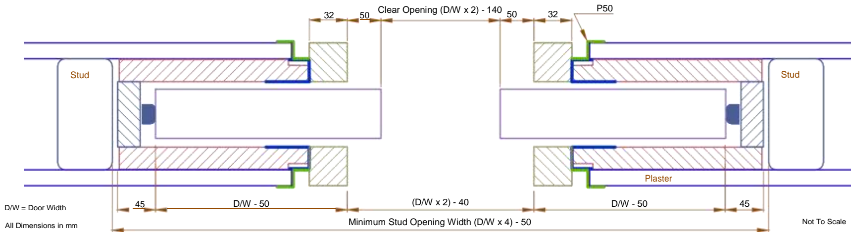
Double Architectural P50 Shadow Line 32mm Reveal (Flush Pull)
